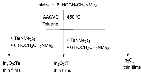
Scheme 5 Deposition of \text{In}_2\text{O}_3 and \text{In}_2\text{O}_3\text{:M} via AACVD.
