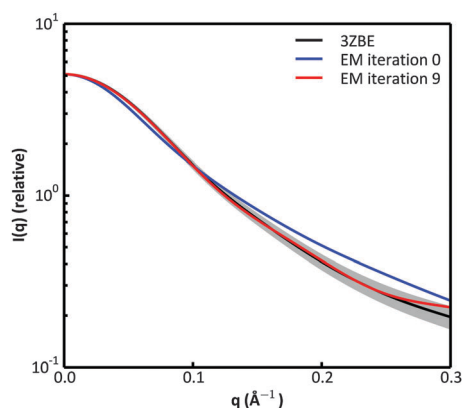
Fig. 3 Scattering curves for the protein PaaA2. The original data calculated from the published structural ensemble are shown in black, with error margins in grey. The fit of the unrestrained ensemble at iteration 0 of the EM algorithm is shown in blue. The fit of the optimized ensemble at iteration 9 of the EM algorithm is shown in red.
