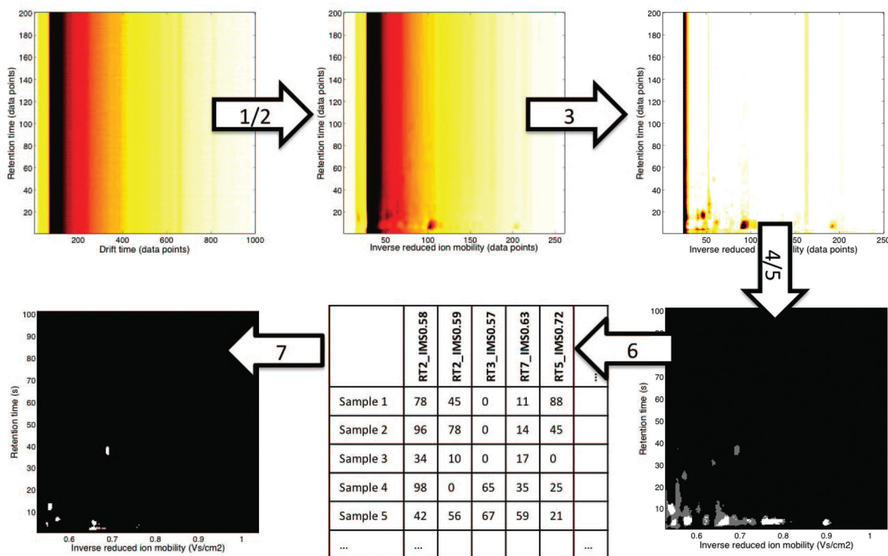
Fig. 3 An example of a non-targeted data analysis strategy for MCC-IMS datasets. 12 It involves the following steps: (1) alignment: correction of drift time to inverse reduced ion mobility values, (2) denoising in RT dimension and 4x compression in IMS dimension with wavelets, (3) baseline correction with top-hat filtering, (4) region selection: RIP region excluded, (5) mask construction: only white and grey regions are included in the further analysis, (6) data unfolding: levels of variables selected during mask construction are reported for all samples, (7) pattern recognition with sparse-PLS-DA on the data matrix obtained in step 6: a classification model with a number of important variables (white regions are important variables).
