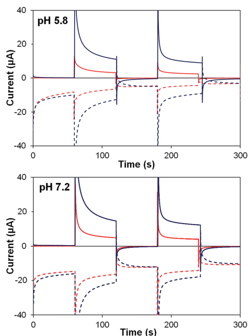
Fig. 6 Photoelectrochemical generator–collector measurements (chronoamperometry) of \text{TiO}_2\text{-P2} (red) and \text{TiO}_2\text{-2} (dark blue) at pH 5.8 and pH 7.2. Solid lines are the photoanode current; dashed lines, collector current; collector efficiency ca. 60%. Applied bias 0 mV vs. Ag/AgCl, illuminated with a 455 nm LED ( 33 \text{ mW cm}^{-2} ). Photocurrent densities are reported in Table 4.
