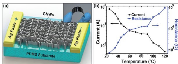
Fig. 3 Thermal response of GNWs/PDMS sensor. (a) Schematic of flexible GNWs/PDMS temperature sensor with a simple structure. The inset shows the optical image of our fabricated temperature sensor prototype. (b) Current and resistance versus temperature curves that range from room temperature ( 25^\circ\text{C} ) to 120^\circ\text{C} by applying a constant voltage of 5 V at the two terminals of the sensor.
