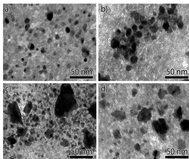
Fig. 8 TEM images of Ni/SiO 2 catalysts with different Ni particle sizes after 150 h on-stream (230 °C, H 2 : CO = 2 : 1, 0.1 MPa). (a) ~8 nm, (b) ~9 nm, (c) ~4 nm, and (d) ~3 nm. Reproduced with permission from ref. 66 Copyright (c) [2014 WILEY-VCH Verlag GmbH & Co. KGaA, Weinheim].
