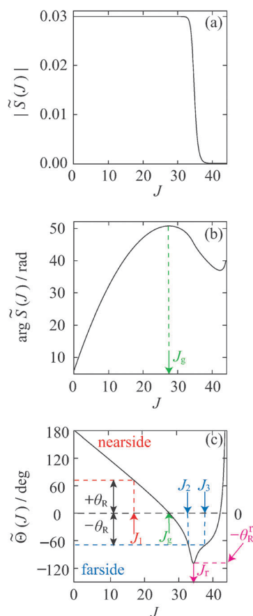
Fig. 2 S matrix data for the J -shifted Eckart parameterization. The values of the parameters are given in Section IV B. (a) |\tilde{S}(J)| versus J . (b) \arg \tilde{S}(J)/\text{rad} versus J . The maximum of the \arg \tilde{S}(J)/\text{rad} curve defines the glory angular momentum variable, J_g , which is indicated by a green dashed line and arrow. (c) \tilde{\Theta}(J)/\text{deg} versus J . The red dashed lines and arrow indicate +\theta_R and J_1 = J_1(\theta_R) for the nearside scattering. The blue dashed lines and arrows indicate -\theta_R , as well as J_2 = J_2(\theta_R) and J_3 = J_3(\theta_R) for the farside scattering. Also shown is the rainbow angular momentum variable, J_r , which is located at the minimum of the \tilde{\Theta}(J)/\text{deg} curve, where \tilde{\Theta}(J) = -\theta_R^f (pink arrow and dashed line respectively), together with J_g , which satisfies the equation \tilde{\Theta}(J_g) = 0 (green arrow).
