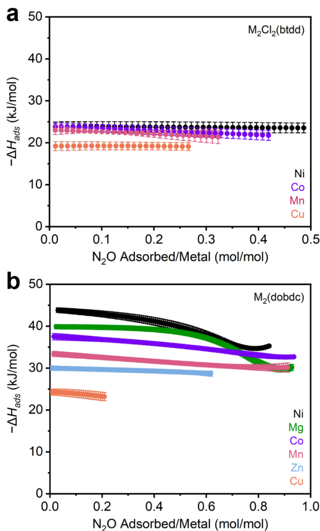
Figure 2. a) -\Delta H_{ads} vs. N 2 O uptake calculated from N 2 O adsorption isotherms in a) M 2 Cl 2 (btdd) (M = Ni, Co, Cu, Mn) and b) M 2 (dobdc) (M = Ni, Mg, Co, Mn, Zn, Cu) MOFs.
