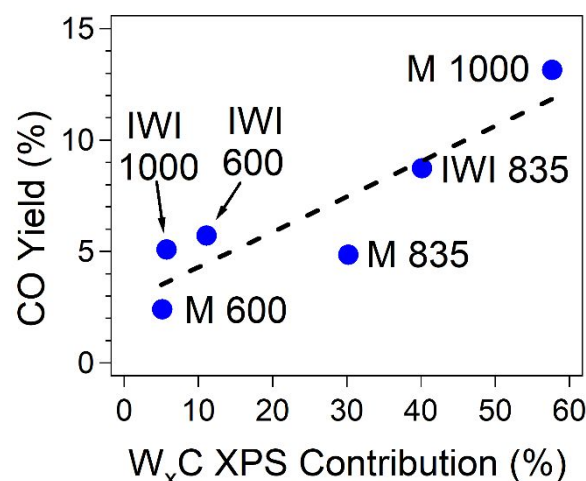
Figure 8. Correlation between RWGS activity and XPS contributions of tungsten carbides ( W_xC ), represented as WC plus W_2C .
