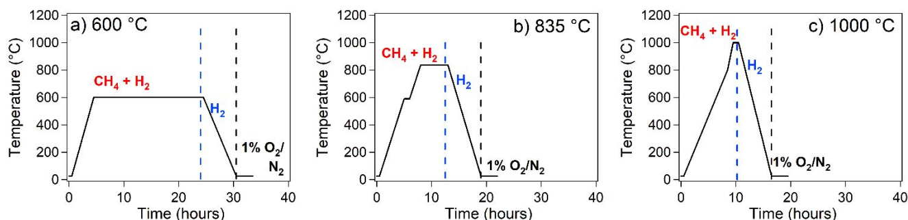
Figure 1. Carburization profiles for M and IWI with a maximum temperature and duration of: a) 600 °C, 20 hours; b) 835 °C, 5 hours; c) 1000 °C, 1 hour.
