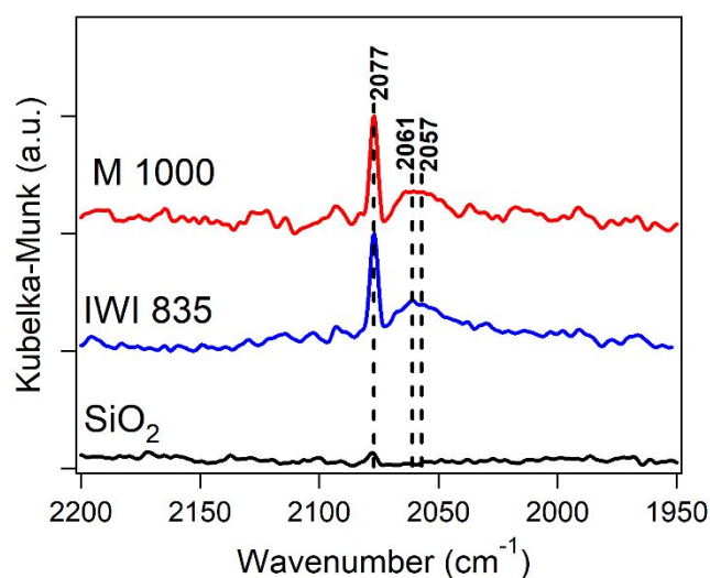
Figure 5. DRIFTS spectra of reduced M 1000, IWI 835 and bare SiO_2 at 25 °C after CO_2 adsorption. The peaks at 2077 cm^{-1} , 2061 cm^{-1} and 2057 cm^{-1} suggest CO_2 is dissociating into CO.
