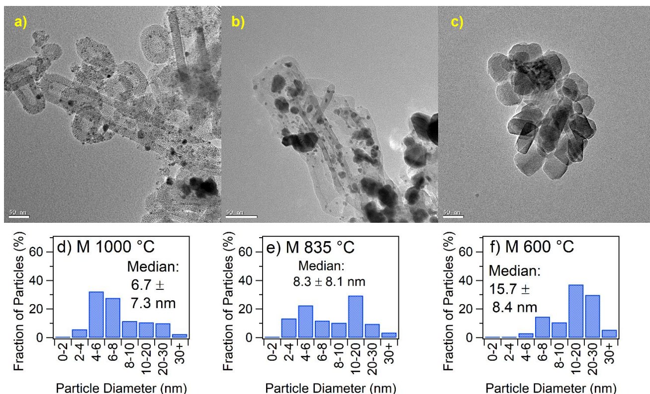
Figure 2. (a-c) TEM images with 50 nm scale bars of nano-W x C (M) carburized at a) 1000 °C, b) 835 °C, and c) 600 °C, with corresponding particle size distributions (d-f).
