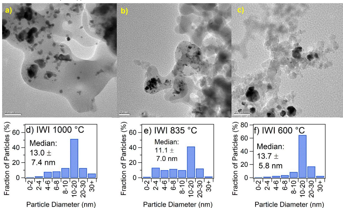
Figure 3. (a–c) TEM images with 50 nm scale bars of IWI W x C carburized at a) 1000 °C, b) 835 °C, and c) 600 °C, with corresponding particle size distributions (d–f).
