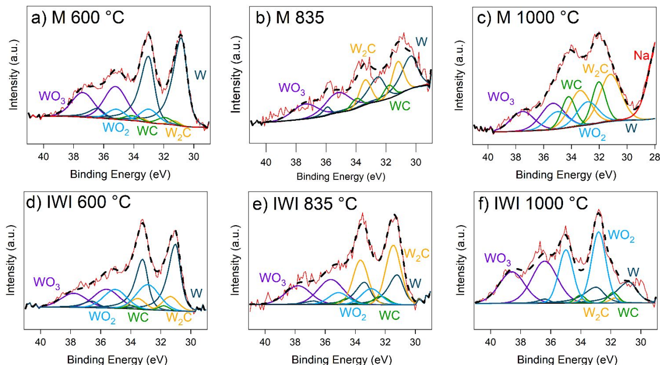
Figure 7. W 4f XPS spectra for W_xC -based catalysts after 12 hours time-on-stream. a) M 600, b) M 835, c) M 1000, d) IWI 600, e) IWI 835 and f) IWI 1000.
