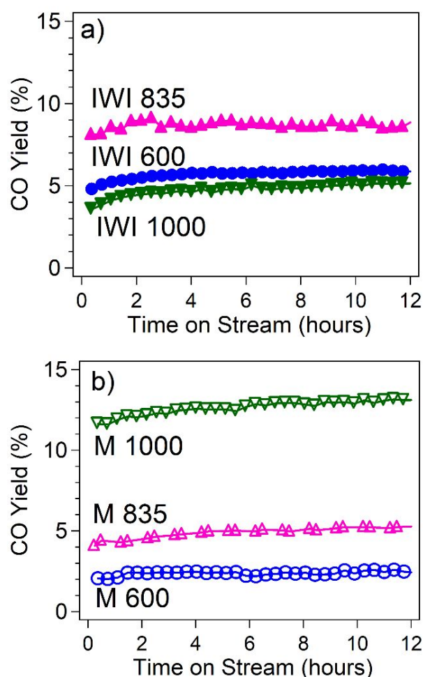
Figure 6. CO yield of \text{W}_x\text{C}/\text{SiO}_2 over 12 hours time-on-stream, synthesized via a) incipient wetness impregnation (IWI), and b) nano- \text{W}_x\text{C} (M). Experiments are conducted at a GHSV of 27,000 mL/h/g with a 3:1 \text{H}_2 : \text{CO}_2 reactant ratio at 350 \text{ }^\circ\text{C} and 2.1 MPa.
