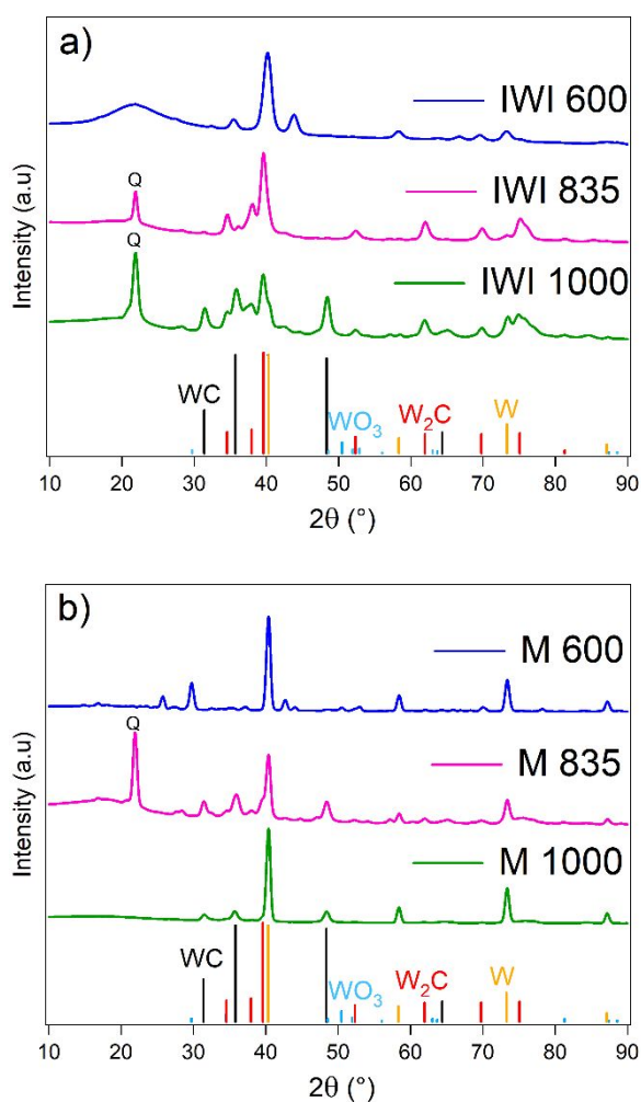
Figure 4. X-ray diffraction patterns of W_xC -based catalysts. a) incipient wetness impregnation (IWI) and b) nano- W_xC (M).
