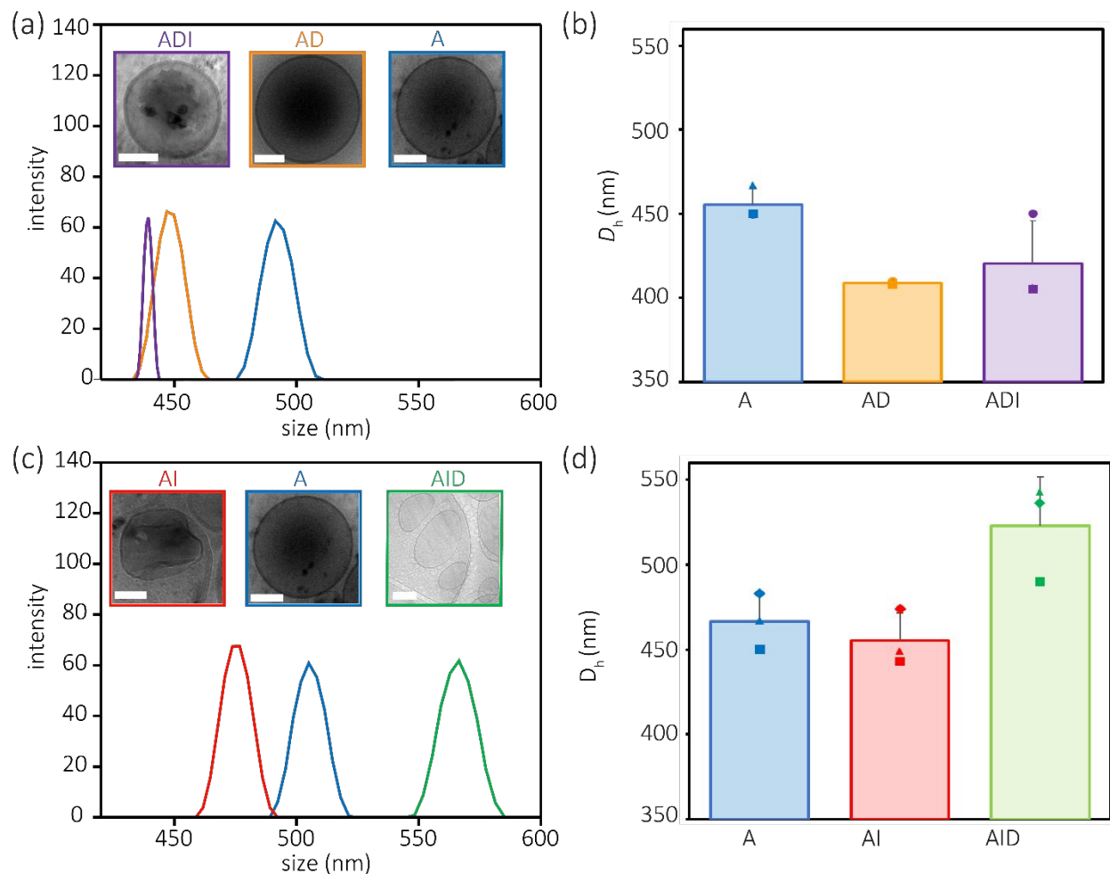
Figure 2. Analysis of the effect of UV-crosslinking, dialysis and combinations thereof on vesicle size and morphology for PEG 45 - b -P(S- stat -CMA) 206 - b -PEG 45 . For each sample, the order of treatments, assembly (A), irradiation with UV (I) and dialysis (D), is represented by that of the corresponding letters. For the dialysis-first sequence, (a) DLS size distributions (at 120°) and corresponding cryo-TEM micrographs (insets) show the change in size of the polymersomes for each treatment while (b) the bar chart shows the variation in the average D_h extracted from the translational diffusion coefficient at multiple angles. For the crosslinking-first sequence, (c) DLS
