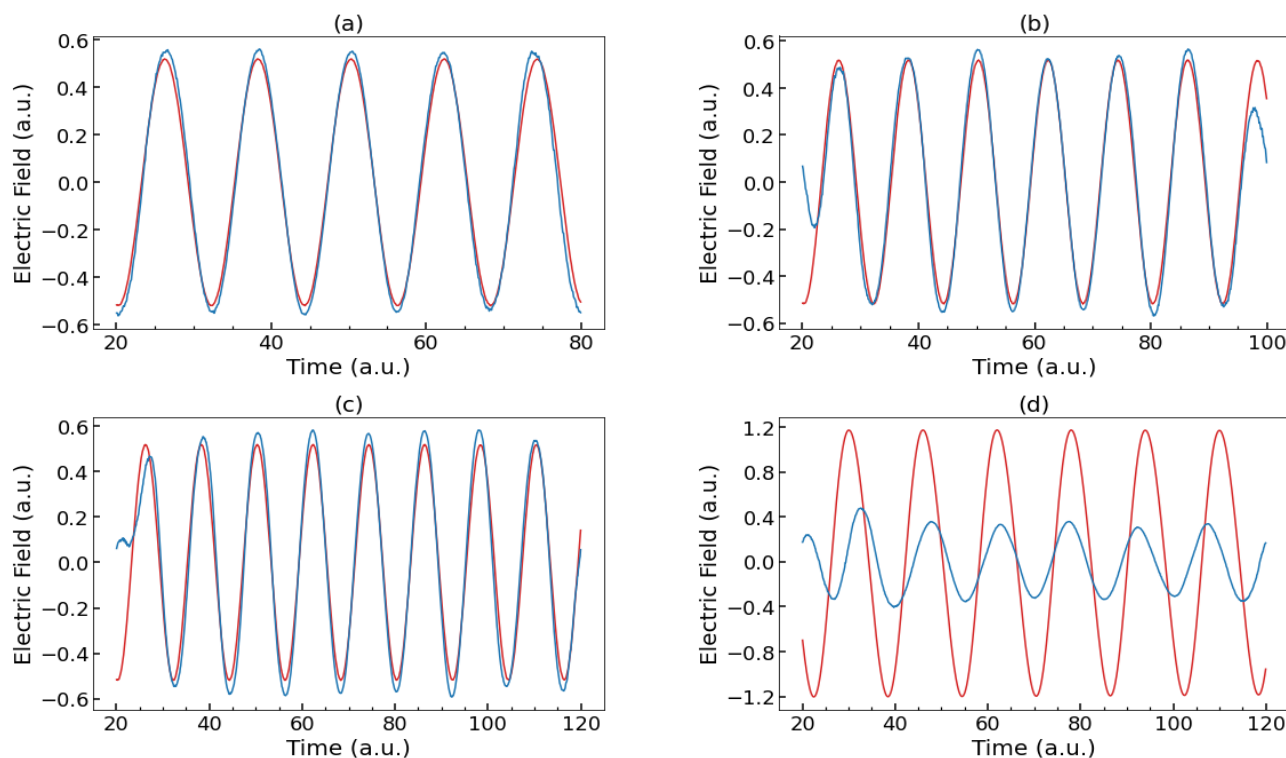
Figure 8: Comparisons of true (red) and machine-learned predicted (blue) E(t) fields. The electric fields correspond to the same potential, but with (a) 600, (b) 800, and (c) 1,000 units. (d) True (red) and machine-learned (blue) E(t) for a different potential characterized by a large amplitude. When the true E(t) has a much larger amplitude, the machine learning algorithm is able to still accurately predict the resonance frequency but underestimates the amplitude.
