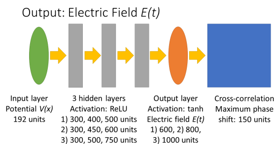
Figure 6: Architecture of the FNN used to predict the electric field, E(t) . The FNN starts with an input layer composed of 192 units (which correspond to the potential, V(x) , evaluated across 192 points), followed by three hidden layers of various sizes. The output layer is composed of 1,000 (or fewer) units and is directly interfaced with a cross-correlation algorithm to predict the final electric field, E(t) .
