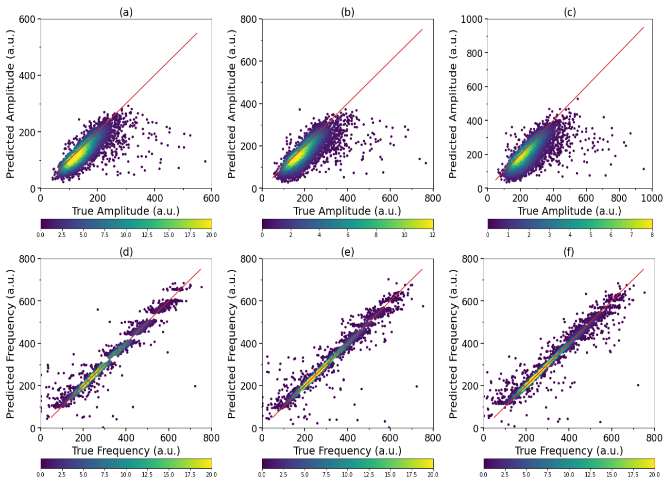
Figure 9: Density plots of the predicted and true amplitude for the (a) 600-, (b) 800-, and (c) 1000-output-layer-unit model, respectively. Density plots of the predicted and true resonance frequency for the (d) 600-, (e) 800-, and (f) 1000-output-layer-unit model, respectively. The diagonal line in each plot represents a perfect match between the machine-learned predictions and true values.
