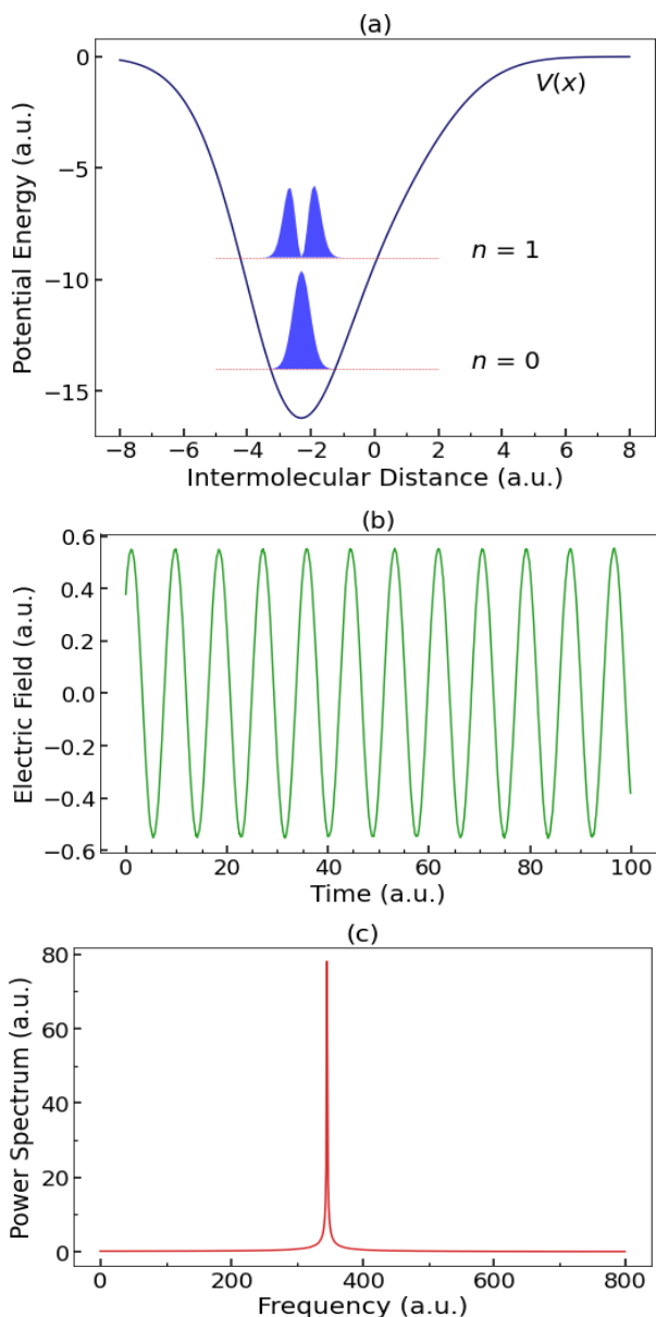
Figure 1: Schematic example of (a) a potential well, V(x) , as a function of intermolecular distance x . The horizontal dashed lines denote the energy levels of the ground and first excited state, and their respective probability wavefunctions, |\psi(x)|^2 , are depicted as blue curves above the energy levels; (b) the optimal electric field E(t) required to excite the transition between the ground and the first excited state; (c) the corresponding power spectrum \sigma(\omega) as a function of frequency \omega , obtained from the fast Fourier transform of E(t) .
