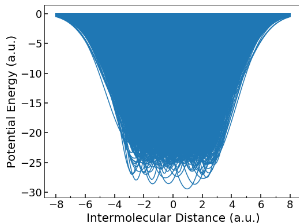
Figure 2: Plot of all 36,118 potentials sampled in this work. The center region of the V(x) space is densely packed and fully sampled, indicating that the full set of these potentials sufficiently explores this phase space. The side regions of the figure are not filled by the potential energy curves since the range of the Gaussian centers, \mu , were intentionally kept small to prevent the wavefunctions from spreading outside the x \in [-8.0, 8.0] range.
