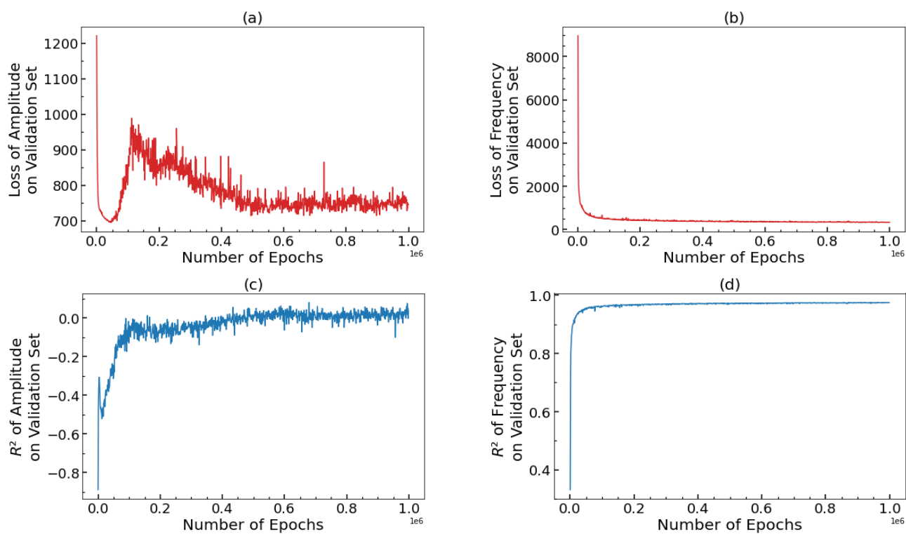
Figure 5: Plot of loss vs. number of epochs for FNN predictions of (a) the amplitude and (b) resonance frequency. R^2 values for the FNN-predicted (c) amplitude and (d) resonance frequency. All plots were generated from the validation dataset.
