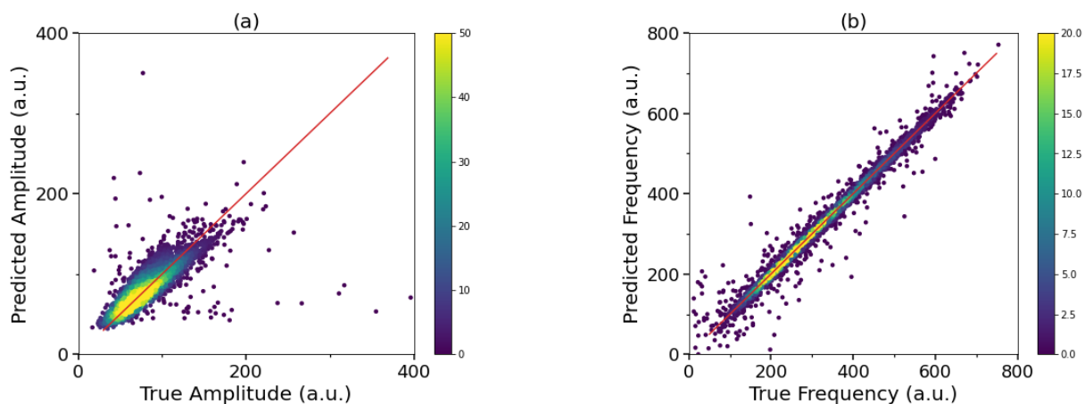
Figure 4: Density plots of the machine-learned predicted vs. true (a) amplitudes and (b) frequencies. The diagonal line in each plot represents a perfect match between the machine-learned predictions and true values. Both plots were obtained with 1,000,000 epochs.
