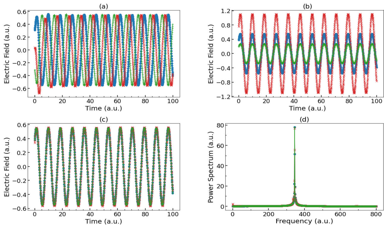
Figure 7: (a) Optimized electric field, E(t) , with various phase shifts, \phi . The blue data points denote the optimized E(t) obtained directly from the NIC-CAGE code. The red curve is the same E(t) with a phase shift of \pi/2 , and the green curve is E(t) with a phase shift of \pi . When each of these electric fields are used as initial guesses for propagating the time-dependent Schrödinger equation, all of them gave a transition probability close to unity (which shows that the transition probability is insensitive to the phase, \phi ). (b) Optimized electric field, E(t) , with various amplitudes. The blue data points denote the optimized E(t) obtained from the NIC-CAGE code, and the red and green curves denote the same E(t) with amplitudes multiplied by 2 and 0.5, respectively. When each of these electric fields were used as initial guesses for time propagation, all of them reverted/converged back to the E(t) with the original amplitude shown in panel (c), which indicates that the transition probability depends critically on the electric field amplitude. (d) Power spectra, \sigma(\omega) , of the various E(t) fields depicted in (a), showing that they coincide with each other, as expected.
