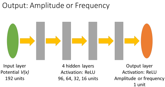
Figure 3: Architecture of the FNN used to predict the amplitude and resonance frequency of the power spectrum, \sigma(\omega) . The FNN starts with an input layer composed of 192 units (which correspond to the potential, V(x) , evaluated across 192 points), followed by four hidden layers of various sizes. The output layer is composed of 1 unit to predict either the amplitude or resonance frequency of \sigma(\omega) .
