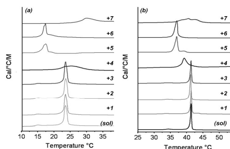
Figure 4. DSC traces of DMPC (a) and DPPC (b) liposomes in pure water or in presence of 1,3,5-triamide cis,cis -cyclohexane derivatives ( 1 , 2 , 3 ), Dibenzoyl cysteine 4 , bis(leucine) oxalyl-amide 5 , Monourea ethyl serine gelator 6 and gemini tartrate surfactant 7 .
