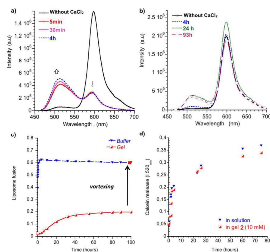
Figure 6. Emission spectra of DOPS vesicles containing 1 mol % fluorescent phospholipids N-NBD-PE and N-Rh-PE before and after the addition of \text{CaCl}_2 (a) in buffer and (b) in a gel network of 2 . (c) DOPS fusion as a function of time in buffer or in a gel of 2 . (d) Calcein release from DOPS vesicles in buffer or embedded in a gel network of 2 , as followed by the progressive increase of the fluorescence at 520 nm.
