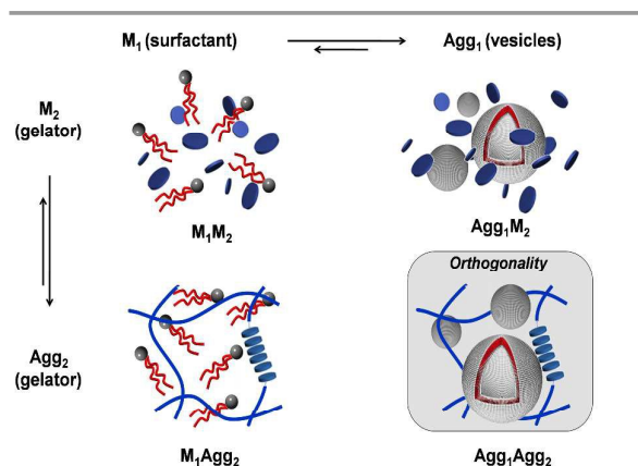
Figure 1. The different aggregation states in a two-component system of phospholipids and hydrogelators. Both gelators and phospholipids can exist in their monomeric state ( M_i ) or aggregated state ( Agg_i ). This scheme represents only orthogonal self-assembly in which components do not interact with each other.
