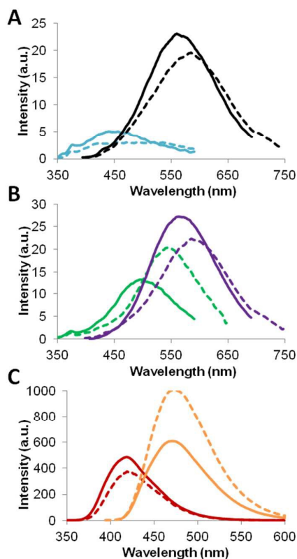
Fig. 5 Emission spectral overlays of duplex (dashed lines) and GQ (solid lines) produced by (A) AcphdG (blue lines) vs. vAcphdG (black lines) at syn-G 5 , (B) AcphdG (green lines) vs. vAcphdG (purple lines) at loop- G 8 and (C) BthdG (red lines) vs. vBthdG (orange lines) at syn-G 5 .
