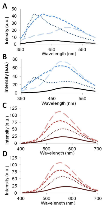
Fig. 6 Emission spectral overlays of AcphdG-mTBA (A and B) and vAcphdG-TBA (C and D) at syn-G 6 (A and C) and loop-G 6 (B and D) in K + solution (solid traces) and in the presence of 42.5% (v/v) CH 3 CN (dotted traces), PEG-200 (dashed traces) and PEG-600 (long dashed traces).
