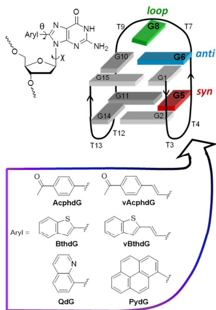
Fig. 1 Structures of 8-aryldG probes and sites of incorporation into TBA (G-tetrad; G5, red, syn ), G6, blue, anti ), and loop region (G8, green). The dihedral angle \chi ( Z(O4'-C1'-N9-C4) ) defines the glycosidic bond orientation to be anti ( \chi = 180 \pm 90^\circ ) or syn ( \chi = 0 \pm 90^\circ ), and \theta ( Z(N9-C8-C10-X11) ) defines the degree of twist between the nucleobase and the 8-substituent.
