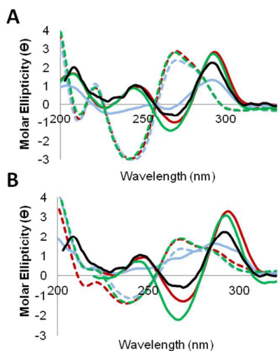
Fig. 4 CD spectral overlays of duplex (dashed lines) and GQ (solid lines) produced by (A) AcphdG-mTBA and (B) BthdG-mTBA; red lines ( syn -G 5 ), blue lines ( anti -G 6 ) and green lines (loop-G 8 ); black trace is GQ spectrum of unmodified TBA.
