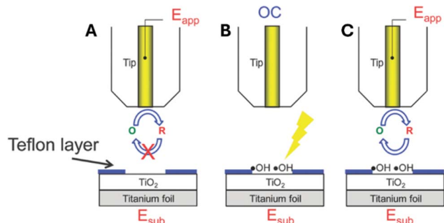
Fig. 3 Photo-SI-SECM operation scheme for the reduction of photogenerated \bullet\text{OH}_{(ads)} on \text{TiO}_2 . (A) No \bullet\text{OH}_{(ads)} is produced in the dark; the substrate surface is inert. (B) Tip is at open circuit, and \bullet\text{OH}_{(ads)} are generated on \text{TiO}_2 through surface irradiation. (C) Light is switched off; tip-generated R species react with \bullet\text{OH}_{(ads)} . Adapted from ref. 21 with permission from Royal Society of Chemistry, copyright 2012.
