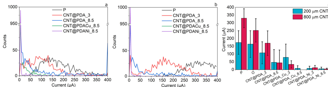
Fig. 5 Distribution of current measured by C-AFM for 200 (a) and 800 (b) \mu\text{m} pristine CTNs, CNTs functionalized with PDA at pH 3 and 8.5, and in the presence of copper and nickel ions. Weighted average current values (c) of 200 and 800 \mu\text{m} pristine and oxidized CNTs, as well as CNTs functionalized with PDA at pH 3 and 8.5, and as well in the presence of copper and nickel ions. Error bars represent the standard deviation from six independent measurements per sample.
