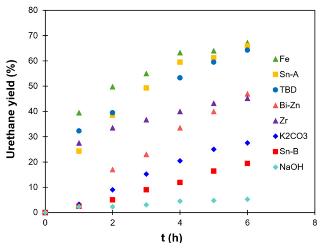
Fig. 2 Kinetic study at 140 °C of the model TU reaction by ^1\text{H} NMR: yield of urethane product depending on the catalyst used.
