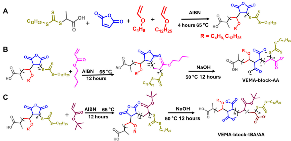
Scheme 1 (A) Synthesis of VEMA copolymers using RAFT copolymerization of vinyl ether and maleic anhydride (B) addition of n -butyl acrylate block in VEMAN and hydrolysis to synthesize VEMA- block -AA polymers (C) addition of tert -butyl acrylate block in VEMAN and hydrolysis to synthesize the mixture of VEMA- block - t BA and VEMA- block -AA polymers.
