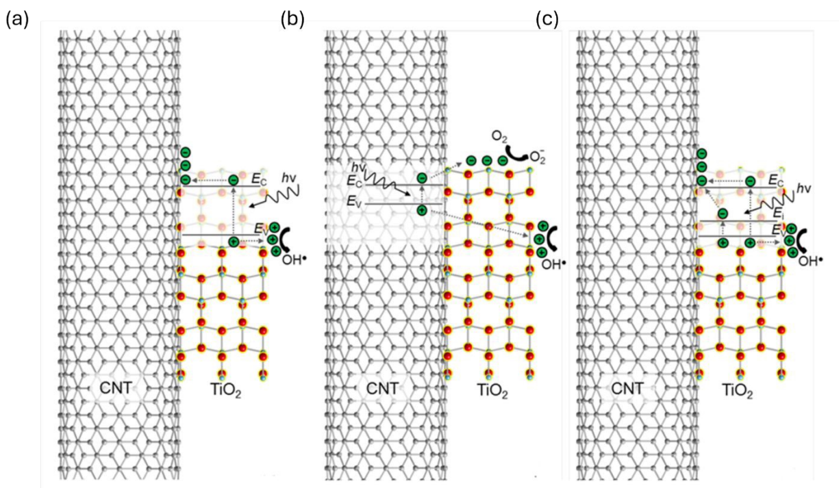
Fig. 11. Mechanism of \text{TiO}_2 -CNT composite. (a) electron scavenging, (b) photosensitization, and (c) band-gap modification 166 . Fig. 11a-c reprinted from 166 Beilstein Journal of Nanotechnology, 5, 946-955, 2014.
