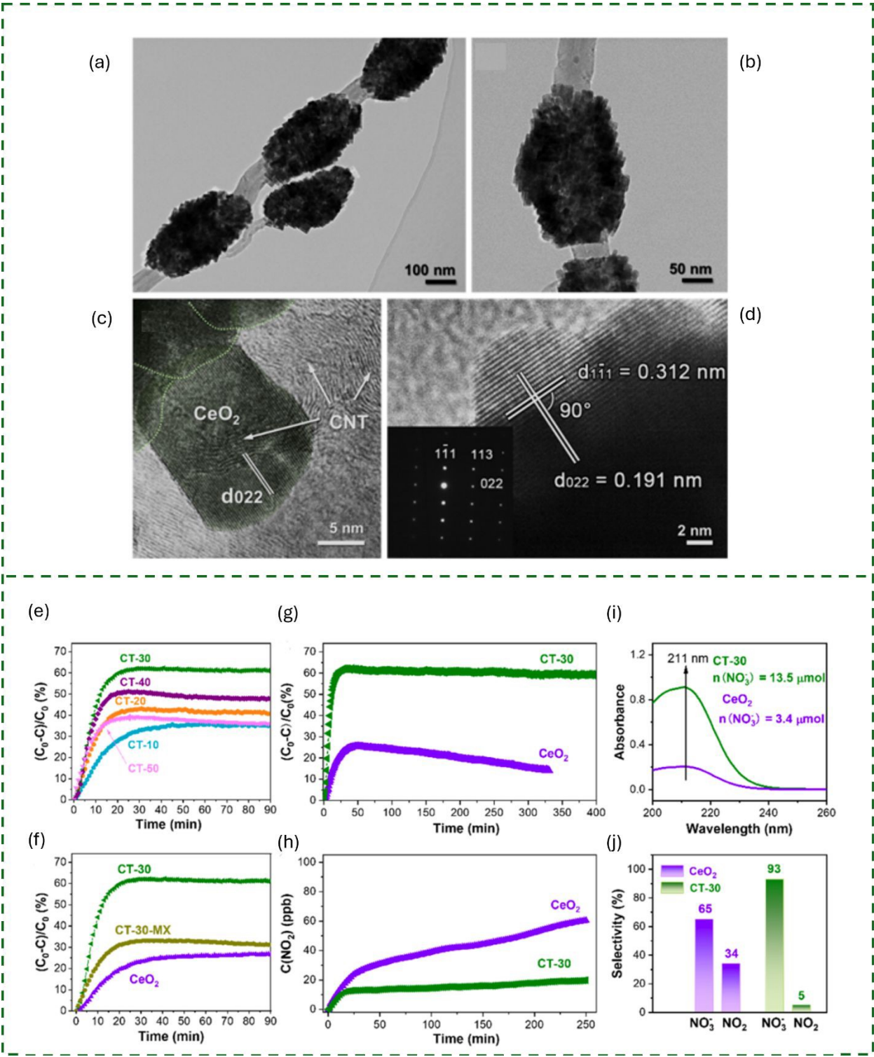
Fig. 13. (a,b) TEM images and (c,d) HRTEM images of CT-30 (the SAED pattern in the inset). Photocatalytic NO oxidation performance of (e) CT-series samples with different CNT contents and (f) \text{CeO}_2 , CT-30, and CT-30-MX, (g) long-term stability test and (h) concentration
