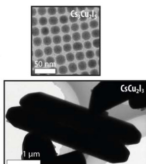
Fig. 12 Caesium copper halides as representative of copper halide SNCs. (a) Unit cell, copper cluster geometry, and simulated XRPD patterns of the most common compositions reported for \text{Cs-Cu-X} (where \text{X} = \text{Cl}, \text{Br}, \text{I} ). (b) Absorption (dashed lines) and emission (solid lines) spectra of \text{Cs}_3\text{Cu}_2\text{I}_5 (blue) and \text{CsCu}_2\text{I}_3 (yellow), alongside a photo of the dispersion under UV excitation, and the corresponding photoluminescence decay curves. Adapted with permission from ref. 286, Copyright 2019, American Chemical Society. (c) The emission stems from a self-trapped exciton. (d) Representation of the Jahn-Teller distortion that occurs after excitation in \text{Cs}_3\text{Cu}_2\text{I}_5 . Adapted with permission from ref. 287, Copyright 2025, Springer. (e) Absorption and emission spectra, photoluminescence decay curves, and photo under UV excitation of a series of alloyed \text{Cs}_3\text{Cu}_2\text{X}_5 SNCs, alongside \text{Cs}_3\text{Cu}_2\text{Cl}_5 SNCs. Adapted with permission from ref. 288, Copyright 2020, American Chemical Society. (f) Scheme of the synthesis protocol for the synthesis of \text{Cs}_3\text{Cu}_2\text{I}_5 SNCs or \text{CsCu}_2\text{I}_3 microcrystals, alongside the TEM images of the respective materials. Adapted with permission from ref. 284, Copyright 2019, John Wiley and Sons. (g) TEM images of \text{Cs}_3\text{Cu}_2\text{I}_5 SNCs obtained using different halide additives, showing optimized morphology and narrow size distribution in the presence of \text{MnI}_2 . Adapted with permission from ref. 289, Copyright 2022, American Chemical Society. (h) TEM images of parent \text{Cs}_3\text{Cu}_2\text{Cl}_5 synthesized at 180^\circ\text{C} and used as sacrificial species for cation exchange with Zn, Bi, and Cd. The TEM images of the SNCs obtained from the cation exchange procedures are reported in the bottom row. Adapted with permission from ref. 290, Copyright 2023, American Chemical Society.
