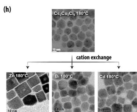
Fig. 12 Caesium copper halides as representative of copper halide SNCs. (a) Unit cell, copper cluster geometry, and simulated XRPD patterns of the most common compositions reported for \text{Cs-Cu-X} (where \text{X} = \text{Cl}, \text{Br}, \text{I} ). (b) Absorption (dashed lines) and emission (solid lines) spectra of \text{Cs}_3\text{Cu}_2\text{I}_5 (blue) and \text{CsCu}_2\text{I}_3 (yellow), alongside a photo of the dispersion under UV excitation, and the corresponding photoluminescence decay curves. Adapted with permission from ref. 286, Copyright 2019, American Chemical Society. (c) The emission stems from a self-trapped exciton. (d) Representation of the Jahn-Teller distortion that occurs after excitation in \text{Cs}_3\text{Cu}_2\text{I}_5 . Adapted with permission from ref. 287, Copyright 2025, Springer. (e) Absorption and emission spectra, photoluminescence decay curves, and photo under UV excitation of a series of alloyed \text{Cs}_3\text{Cu}_2\text{X}_5 SNCs, alongside \text{Cs}_3\text{Cu}_2\text{Cl}_5 SNCs. Adapted with permission from ref. 288, Copyright 2020, American Chemical Society. (f) Scheme of the synthesis protocol for the synthesis of \text{Cs}_3\text{Cu}_2\text{I}_5 SNCs or \text{CsCu}_2\text{I}_3 microcrystals, alongside the TEM images of the respective materials. Adapted with permission from ref. 284, Copyright 2019, John Wiley and Sons. (g) TEM images of \text{Cs}_3\text{Cu}_2\text{I}_5 SNCs obtained using different halide additives, showing optimized morphology and narrow size distribution in the presence of \text{MnI}_2 . Adapted with permission from ref. 289, Copyright 2022, American Chemical Society. (h) TEM images of parent \text{Cs}_3\text{Cu}_2\text{Cl}_5 synthesized at 180^\circ\text{C} and used as sacrificial species for cation exchange with Zn, Bi, and Cd. The TEM images of the SNCs obtained from the cation exchange procedures are reported in the bottom row. Adapted with permission from ref. 290, Copyright 2023, American Chemical Society.
