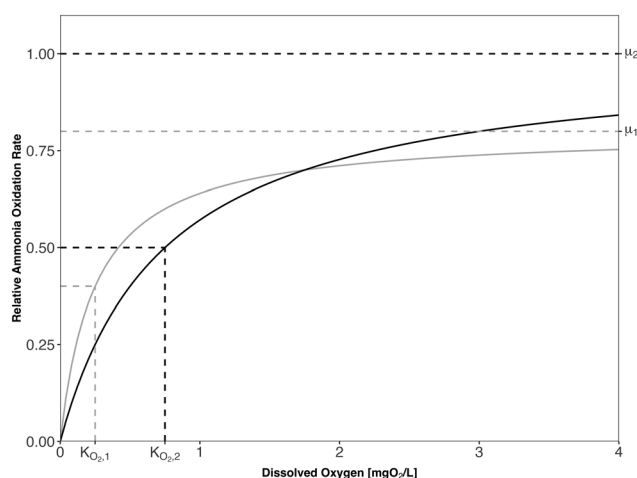
Fig. 1 Two theoretical Monod functions showing ammonia oxidation rate as a function of oxygen with different maximum rates ( \mu_1 and \mu_2 ) and K_{\text{O}_2} ( K_{\text{O}_2,1} and K_{\text{O}_2,2} ).
