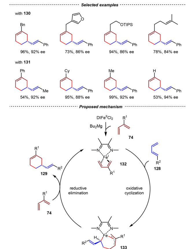
Scheme 29 Fe(I)/ \alpha -diimine-catalyzed asymmetric cross-[4+2] cycloadditions of unactivated 1,3-dienes.
