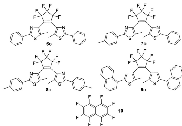
Fig. 8 Photodeformable DAE crystals were grown from 6o , 14 and co-crystals of 7o and 8o , 64 and also from co-crystals of 9o and 10 . 65
