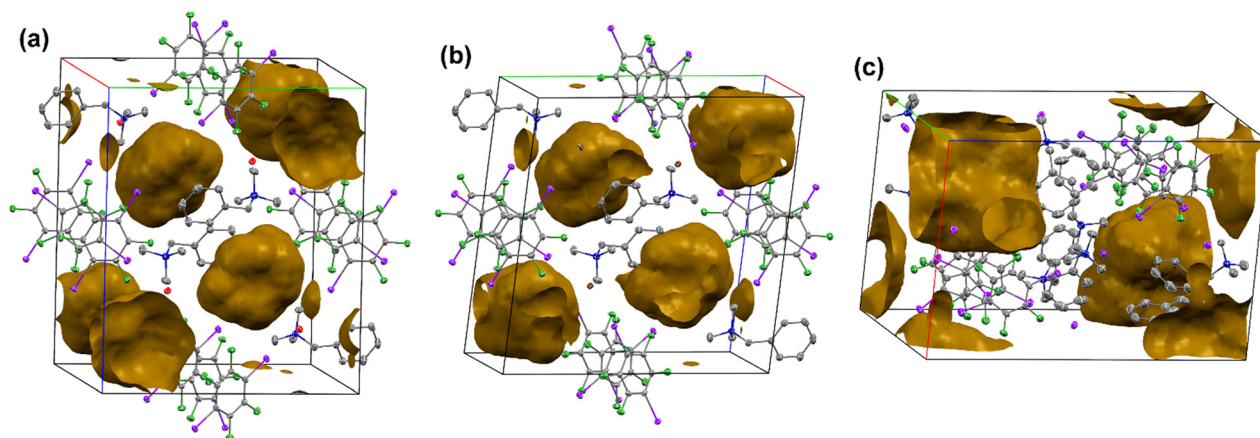
Fig. 6 Solvent voids in \text{NMe}_3\text{BzCl}:\text{p-F}_4\text{DIB}:\text{Ac} (a), \text{NMe}_3\text{BzBr}:\text{p-F}_4\text{DIB}:\text{Ac} (b), and 4(\text{NMe}_3\text{BzI}):4(\text{p-F}_4\text{DIB}):3(\text{Ac}) (c). The a axis is red, the b axis is green, and the c axis is blue.
