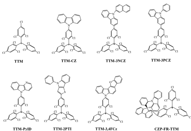
Fig. 8 Typical TTM radicals mentioned in the text.
