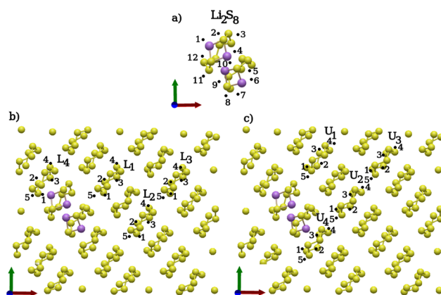
Fig. 7 Third lithiation step: distinct positions on the (001) \alpha -sulfur surface considered for the third lithiation reaction, (a) around Li 2 S 8 dimer obtained in the previous lithiation step, (b) on the lower layers, and (c) on the upper layers around the dimer.
