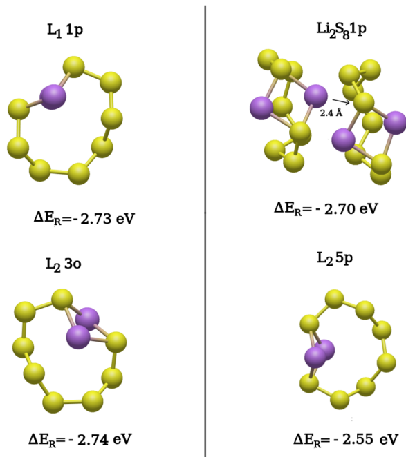
Fig. 6 Second lithiation step: comparison of the lowest-reaction energy structures formed on the lower (left) and the upper (right) sulfur layers. Li 2 S 8 1p refers to the product of the lithiation reaction on an adjacent sulfur ring to the already lithiated one. The others are isolated rings.
