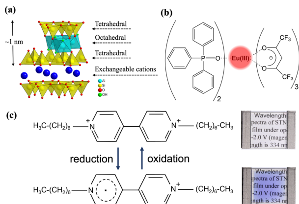
Fig. 1 Chemical structure of (a) smectite, (b) \text{Eu(hfa)}_3(\text{TPPO})_2 , and (c) \text{HV}^{2+} .
