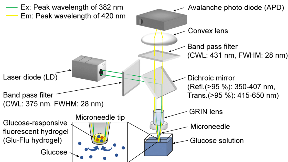
Fig. 4 Schematic diagram of the optical system for D-glucose sensing. The excitation light was focused onto the microneedle tip functionalized with Glu-Flu hydrogel. The microneedle tip was immersed into the D-glucose solution. The fluorescence light from Glu-Flu hydrogel was detected by APD.
