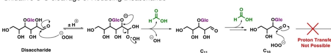
Scheme 3 Plausible mechanisms in the degradation of cellobiose in the presence of a hydroperoxy anion. The absence of C10 disaccharide and the rapid and full conversion to formate argue for a central role of Baeyer–Villiger oxidation.
