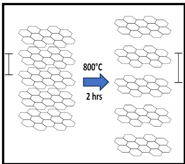
Fig. 9 Schematic of change in interplanar spacing of the active material upon thermal treatment.
