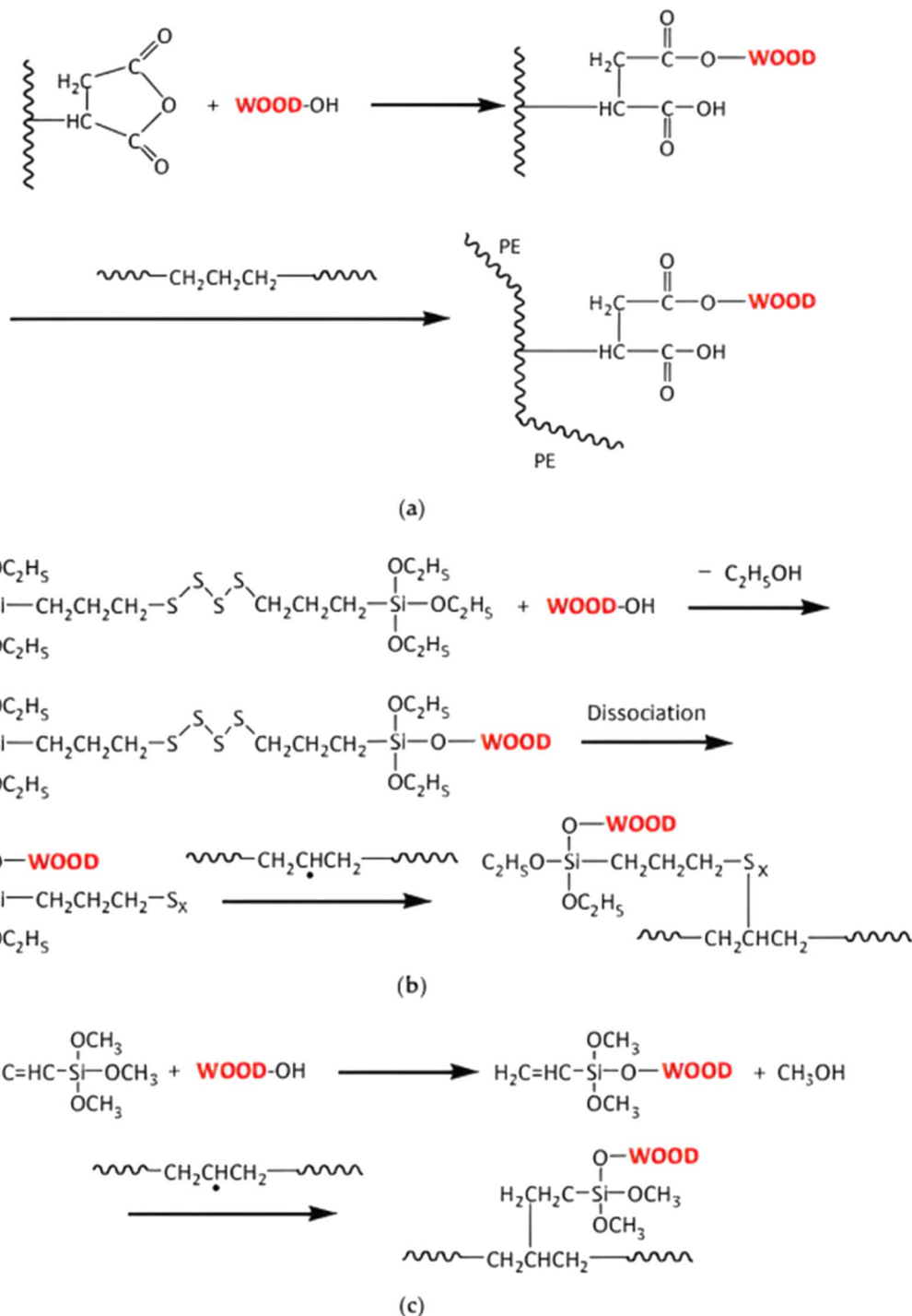
Fig. 7 Possible reactions of coupling agents: (a) MAPE, (b) Si69 and (c) VTMS with wood fibres. Reprinted with permission. 76 Copyright 2018, MDPI.
