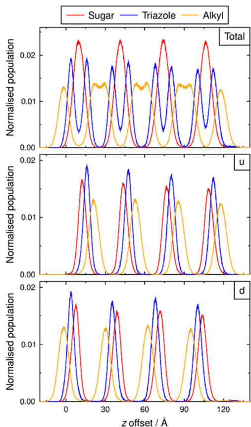
Fig. 11 Normalised populations of sugar (red), triazole (blue) and alkyl (orange) sets of atom centres, taken by averaging over 50–100 ns from the MD simulation of 5 at 40 K below T_{\text{c, sim}} , and showing atom sets from all of the molecules (top), and separately from the two different general forms (u and d).
