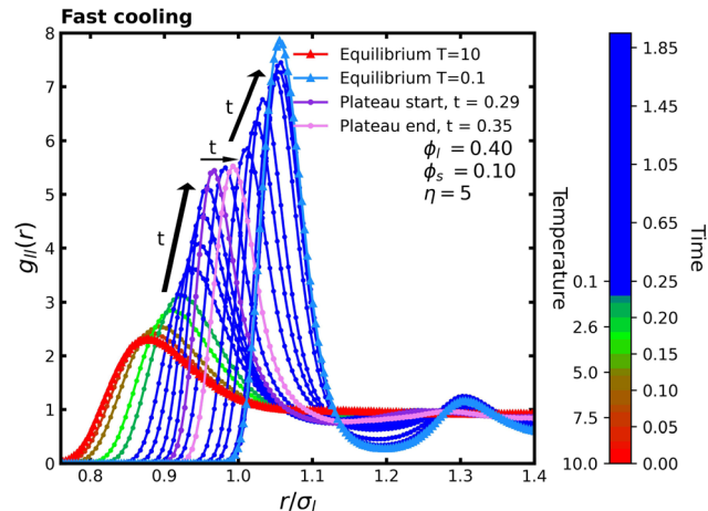
Fig. 6 Evolution of the RDF between large particles ( g_{ll}(r) ) for packing fractions \phi_l = 0.40 and \phi_s = 0.10 with size ratio \eta = 5 , cooled from T_0 = 10 to T_f = 0.1 with a cooling time t_{\text{ramp}} = 0.25\tau_{\text{ref}} . The color bar represents the temperature and time corresponding to each color. Multiple blue curves are shown as the colloidal system continues to evolve after reaching the final temperature.
