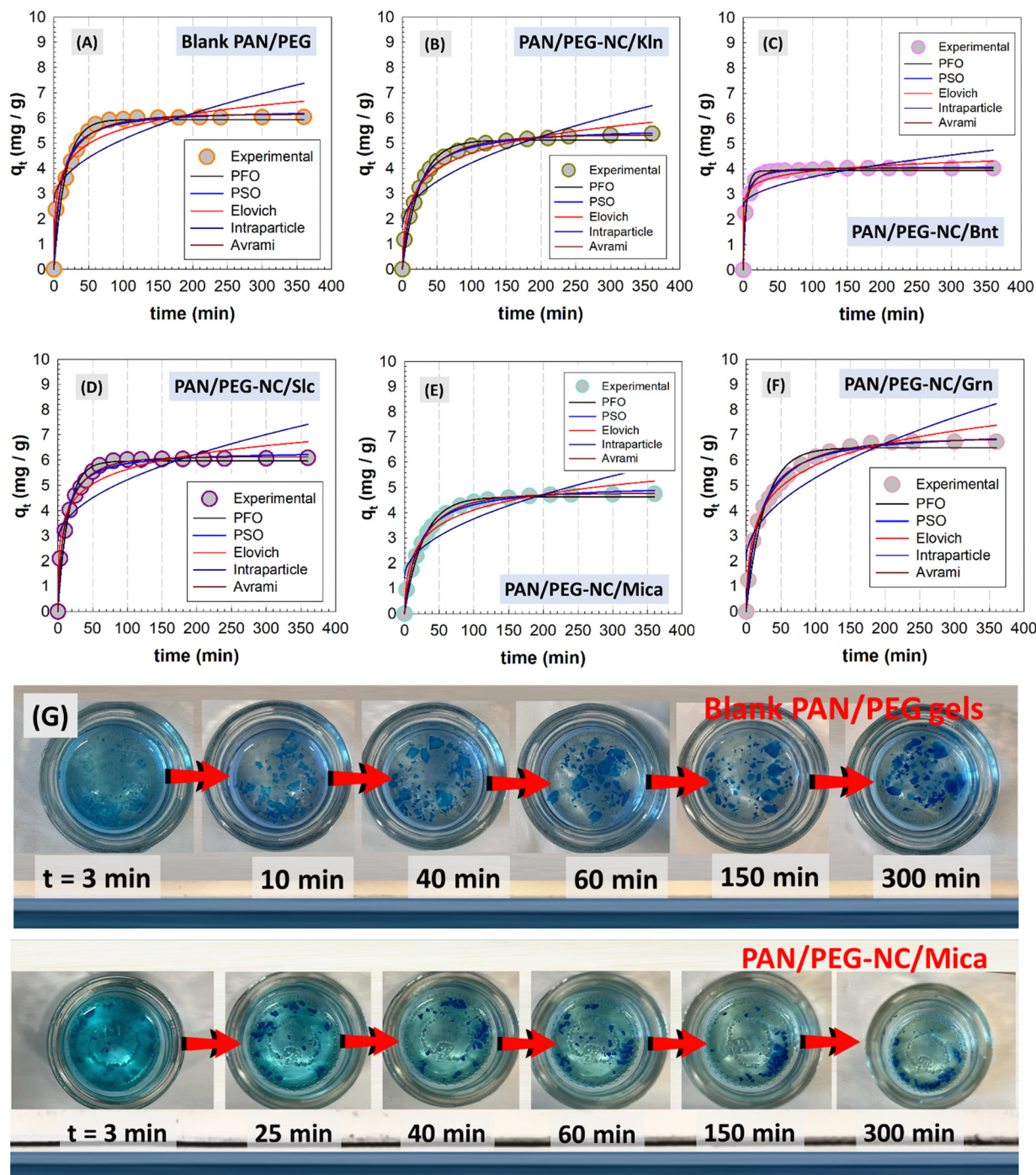
Fig. 9 Results of non-linear PFO, PSO, Elovich kinetic model, intraparticle diffusion model and Avrami kinetic model of blank PAN/PEG and (A) and hybrid PAN/PEG-NC gels containing KIn (B), Bnt (C), Slc (D), Mica (E) and Grn (F). Optical views of blank PAN/PEG and mica-doped PAN/PEG-NC/Mica gels during adsorption (G).
