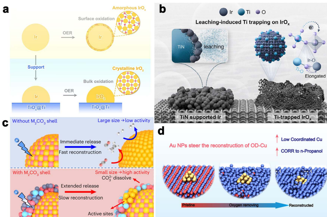
Fig. 5 (a) Schematic illustration of the electrochemically induced reconstruction process of Ir nanoparticles, contrasting scenarios with and without a TiO x @Ti substrate. Reproduced with permission. 90 Copyright 2025, Springer Nature. (b) Schematic illustration of leaching of Ti from a TiN support contributes to a trapping mechanism that stabilizes amorphous IrO x species during the OER. Reproduced with permission. 117 Copyright 2025, Wiley-VCH GmbH. (c) Comparative schematic depicting the projected structural reconstruction pathways of unmodified CuO and carbonate-coated CuO during electrochemical CO 2 reduction. Reproduced with permission. 118 Copyright 2025, Springer Nature. (d) Transformation of CuO into undercoordinated Cu sites localized near Au nanoparticles during CO electroreduction. Reproduced with permission. 119 Copyright 2024, American Chemical Society.
