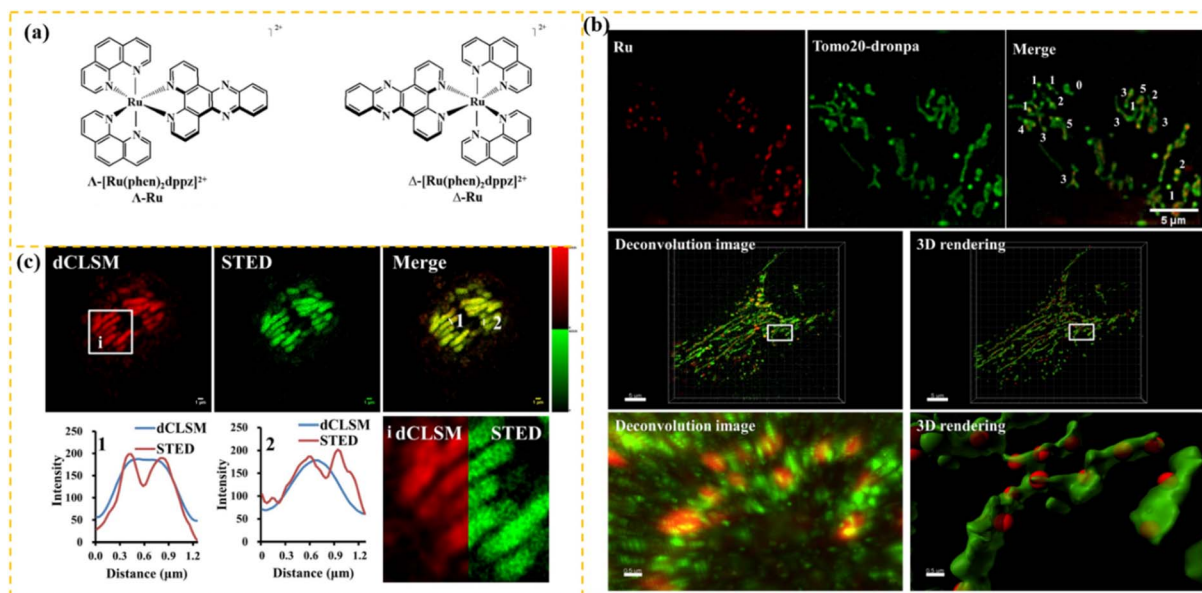
Fig. 23 (a) Enantiomeric structure of compound [\text{Ru}(\text{phen})_2\text{dppz}]^{2+} \text{Cl}_2 . (b) SIM imaging in cellular mitochondria using compound [\text{Ru}(\text{phen})_2\text{dppz}]^{2+} \text{Cl}_2 with the commercial dye Tomo20-dronpa. (c) CLSM and STED imaging of [\text{Ru}(\text{phen})_2\text{dppz}]^{2+} \text{Cl}_2 within living cells. Reprinted with permission from Oxford, copyright 2023, as cited in ref. 78.
