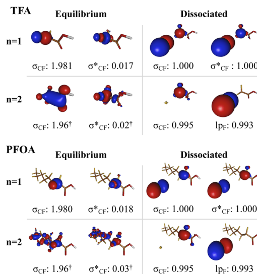
Fig. 4 Natural orbitals and occupation numbers of the dissociated \sigma_{\text{CF}} bond in TFA and PFOA at n = 1 and 2 . Orbital spaces are mixed at n = 2 due to the correlation of more than one orbital at a time at n > 1 , leading to a fully delocalized \sigma_{\text{CF}} space in the equilibrium geometry. For brevity, only one of these delocalized \sigma_{\text{CF}} NOs are shown and their occupation numbers are the average across the NOs exhibiting this bond (indicated by the \dagger symbol). The difference in appearance of singly occupied NOs between n = 1 and 2 is a result of different \pm combinations of electron densities, where the former appears as a \sigma/\sigma^* pair and the latter as a p/\text{lp} pair.
