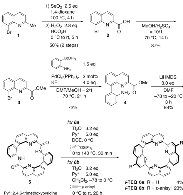
Scheme 1 Synthesis of i -TEQ 6a , 6b .
