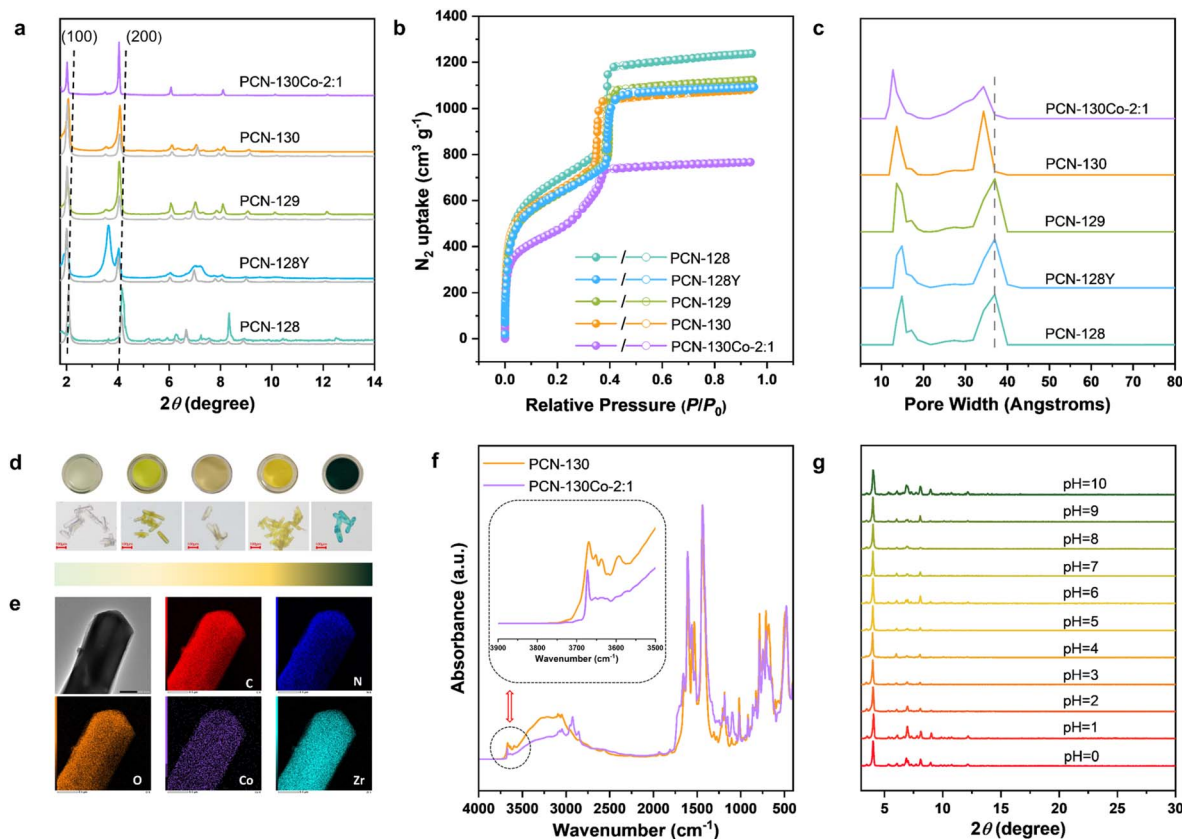
Fig. 2 (a) Simulated and PXR patterns and (b) N_2 adsorption isotherms at 77 K of PCN-128, PCN-128Y, PCN-129, PCN-130, and PCN-130Co-2:1. (c) Pore size distribution of synthesized samples derived from N_2 adsorption isotherms. (d) Pictures and microscope images of PCN-128, PCN-128Y, PCN-129, PCN-130, and PCN-130Co-2:1. (e) TEM image of PCN-130Co-2:1 and corresponding element mapping. (f) The DRIFTS spectra of PCN-130 and PCN-130Co-2:1. Inset: the intensity decay of Zr-OH in the region from 3900 to 3500 cm^{-1} . (g) Stability test of PCN-130Co-2:1 in aqueous solution of pH 0–10 for 12 h.
