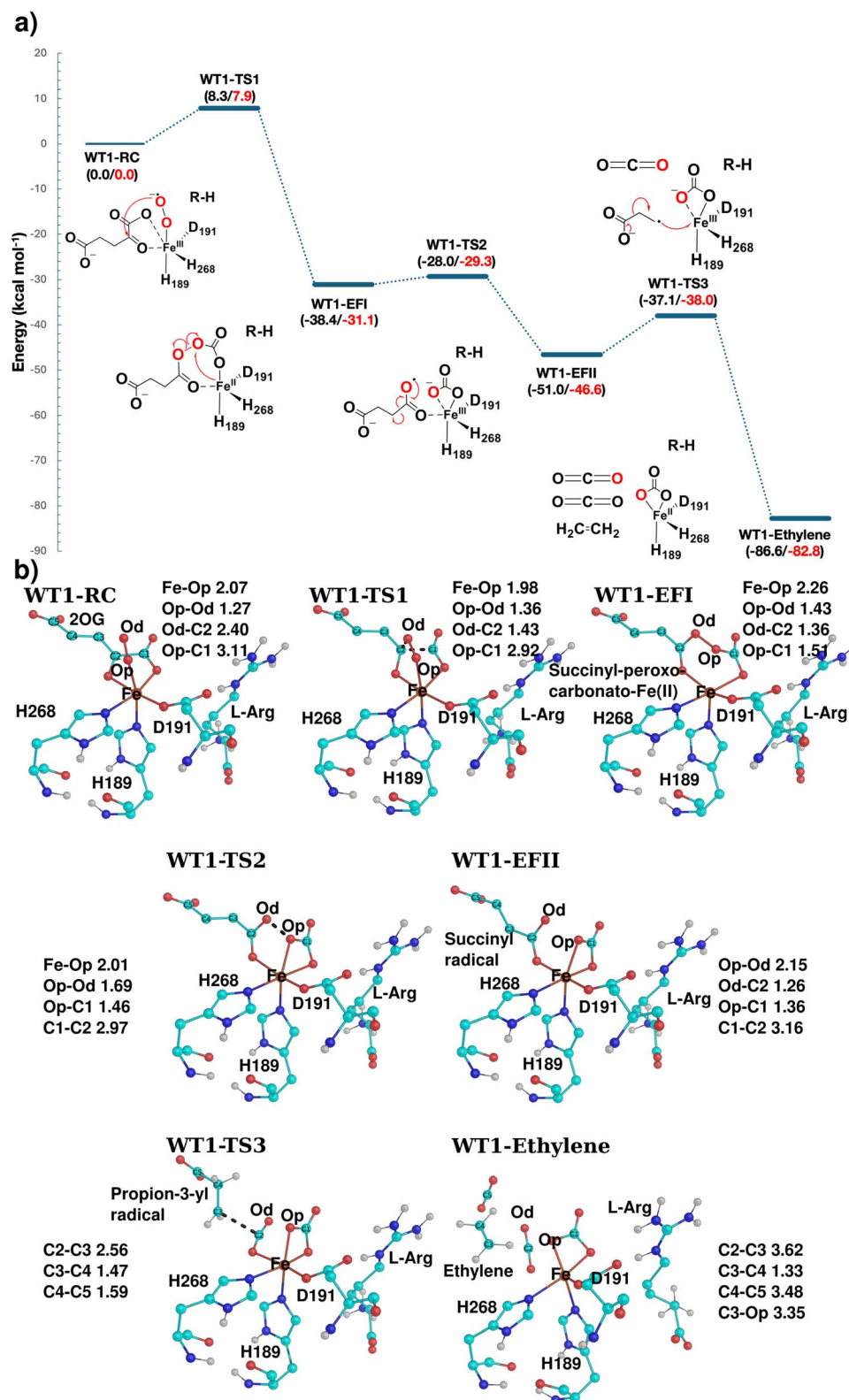
Fig. 3 (a) Reaction profile of the \text{O}_2 activation mechanism from the WT1 snapshot. Relative energies are given in \text{kcal mol}^{-1} at QM(B2)/MM (black) and QM(B3)/MM (red) levels. The profile was plotted at QM(B3)/MM levels. (b) Representations of QM/MM optimized structures obtained during the \text{O}_2 activation mechanism from the EFE WT1 snapshot. Non-polar hydrogens are hidden for clarity. Distances are mentioned in Å.
