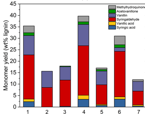
Fig. 13 Gas chromatogram and phenolic monomer yield of the lignin-oil produced from alkaline oxidation of red oak. (a): Reaction conditions 170 °C, 40 psi oxygen, 19.2 wt% catalyst, 1.25 M NaOH, 32 min, (b): reaction conditions are summarized in Table 3.
