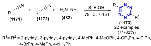
Scheme 325 Synthesis of 1,2,4,5-tetrazines catalyzed by elemental sulfur.
