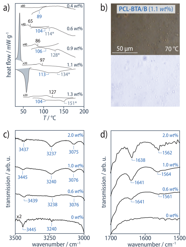
Fig. 5 (a) DSC heating and cooling scans ( 10^{\circ}\text{C min}^{-1} , exothermal transitions up) from PCL-BTA/B blends. For clarity, the PCL melting and crystallization transitions at T_m = 58^{\circ}\text{C} and T_c = 35^{\circ}\text{C} , respectively, are only shown for one composition. (b) Cross-polarized (top) and bright-field (bottom) optical micrographs of PCL-BTA/B recorded at T < T_{\text{agg}} during cooling at 10^{\circ}\text{C min}^{-1} from the melt state. PCL-BTA/B blends at w_B \leq 1.1 wt% remain optically homogeneous (see also ESI Fig. S12 ^{\dagger} ), but ATR FTIR spectra of PCL-BTA/B recorded at 25^{\circ}\text{C} contain (c) the N–H stretching band and (d) the C=O stretching band and the combined N–H bending/C–N stretching band indicative of BTA aggregates at all B concentrations investigated. The sharp absorption signal visible in all the spectra at 3435\text{--}3445\text{ cm}^{-1} is assigned to water absorbed by PCL. 92
