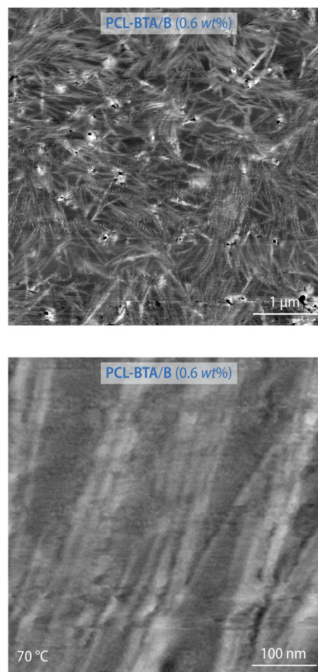
Fig. 6 Intermittent-contact AFM phase images of PCL-BTA/B (0.6 wt%) recorded at 70^{\circ}\text{C} at different magnifications. See ESI Fig. S13 ^{\dagger}
