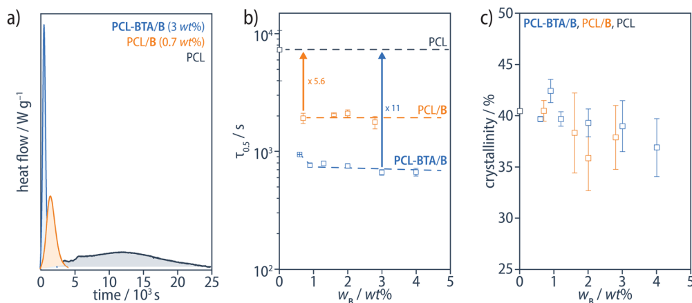
Fig. 11 (a) Examples of isothermal DSC traces for PCL-BTA/B (blue), PCL/B (orange) and pristine PCL (grey) at 48 °C after cooling from 200 °C at 10 °C min -1 to 70 °C, followed by rapid cooling to 48 °C, from which (b) the crystallization half times, \tau_{1/2} , have been determined. \tau_{1/2} is decreased by a factor of up to 5.6 in PCL/B (orange), and up to 11 in blends of PCL-BTA/B (blue) compared with pristine PCL (grey). The dashed curves serve as guides to the eye. (c) The degree of crystallinity of the PCL matrix, as determined by integrating the PCL melting peak in heating scans at 10 °C min -1 recorded immediately after the isothermal step, assuming the melting enthalpy of an ideal PCL crystal to be 139.5 J g -1 . 95
