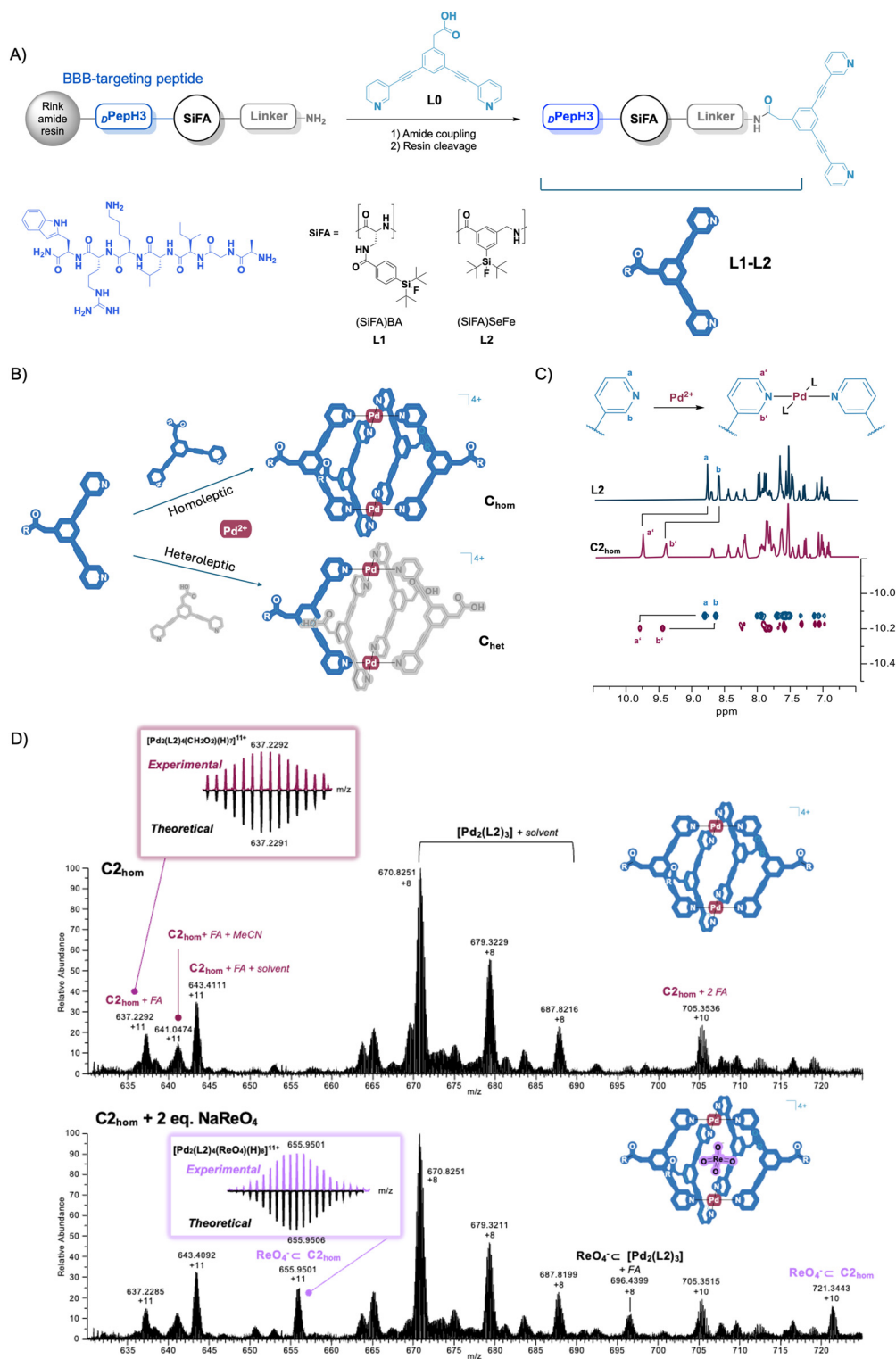
Fig. 2 (A) Design and synthesis of BBB-targeted ligands L1 and L2 by Fmoc-SPPS. The exo-functionalization consists of a BBB shuttle peptide pPepH3 , a silicon-based fluoride acceptor (SiFA) for radiolabeling with the PET nuclide fluoride-18 and a PEG linker (4-((2-(2-(2-aminoethoxy)ethoxy)ethyl)amino)-4-oxobutanoic acid) that acts as a spacer. (B) Coordination-driven self-assembly of homoleptic and heteroleptic MCgs, C_{hom} and C_{het} . Reaction conditions: 4 eq. ligand (in total), 2 eq. [Pd(MeCN)_4](BF_4)_2 , DMSO, RT, 1 h. (C) ^1H NMR (top) and ^1H -DOSY NMR (bottom) spectra in DMSO- d_6 (400 MHz) of C_{2hom} (purple) compared to L2 (blue). The \alpha -pyridinyl protons a and b shift upon metal coordination as explained by the scheme. (D) Mass spectra of C_{2hom} (top) and the host-guest complex ReO_4^- \cdot C_{2hom} (bottom) obtained by DI-HR-ESI-MS. Corresponding theoretical and experimental isotopic patterns are shown in the graph insets.
