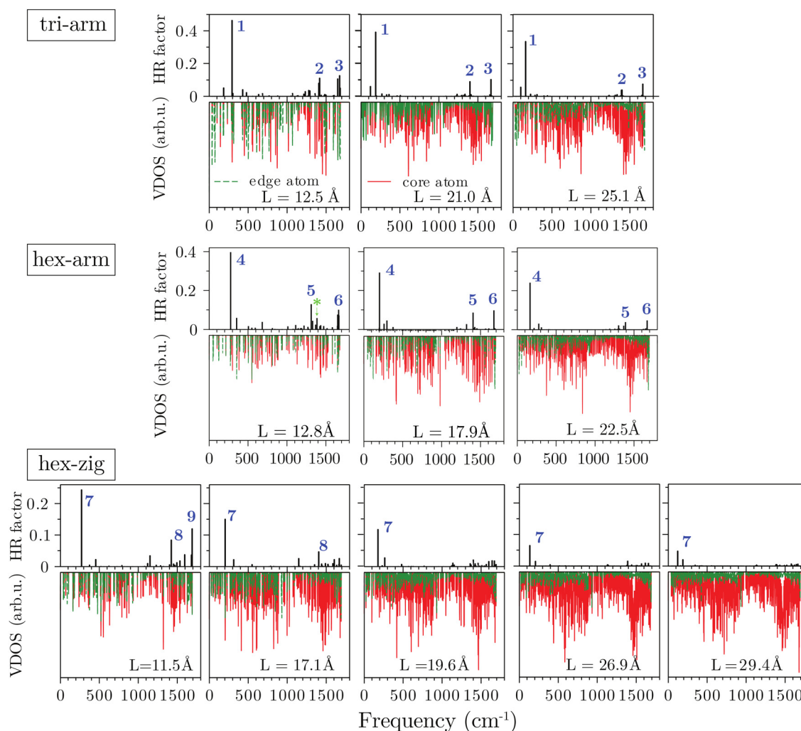
Fig. 5 Frequency-dependent partial HR factors S_i (upper panels) and the VDOSs (lower panels) of the GQDs. From top to bottom shows the tri-angular GQDs with armchair edges, the hexagonal GQDs with armchair edges, and the hexagonal GQDs with zigzag edges. The numbers above the dominant peaks refer to the numbers in Table 2.
