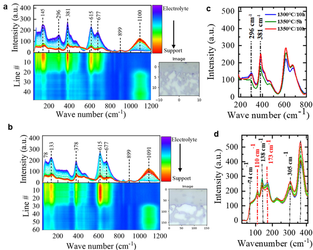
Fig. 7 Line averaged Raman spectra obtained from mapped areas of polished cross-sections of (a) BSZY44362|NiO-SZCY541 half-cell sintered at 1300 °C for 10 hours. (b) Polished cross-section of the half-cell sintered at 1350 °C for 5 hours the optical images. (c) Raman spectra from the electrolyte layer only, highlighting the well-resolved Y-O mode at 296 cm -1 . (d) Raman spectra from the polished cross-section of the half-cell sintered at 1400 °C.
