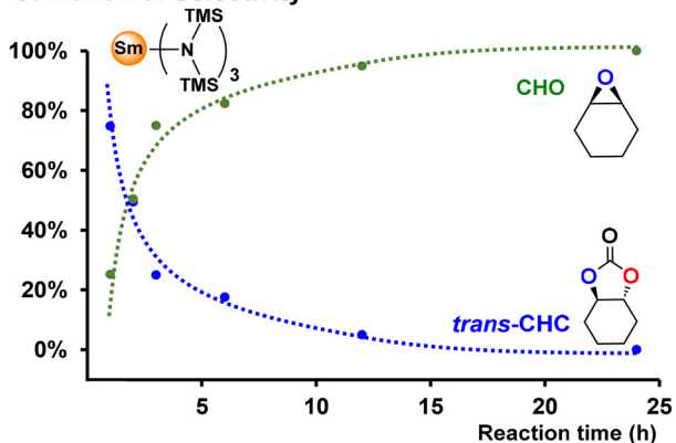
Fig. 1 A. Kinetic profile of PCHC depolymerization in a closed reaction system using \text{La}^{\text{NTMS}} under the conditions of Table 1. B. Total monomer conversion ( trans -CHC + CHO) versus reaction time. C. Kinetic profile of PCHC depolymerization in a closed reaction system using \text{Sm}^{\text{NTMS}} .
