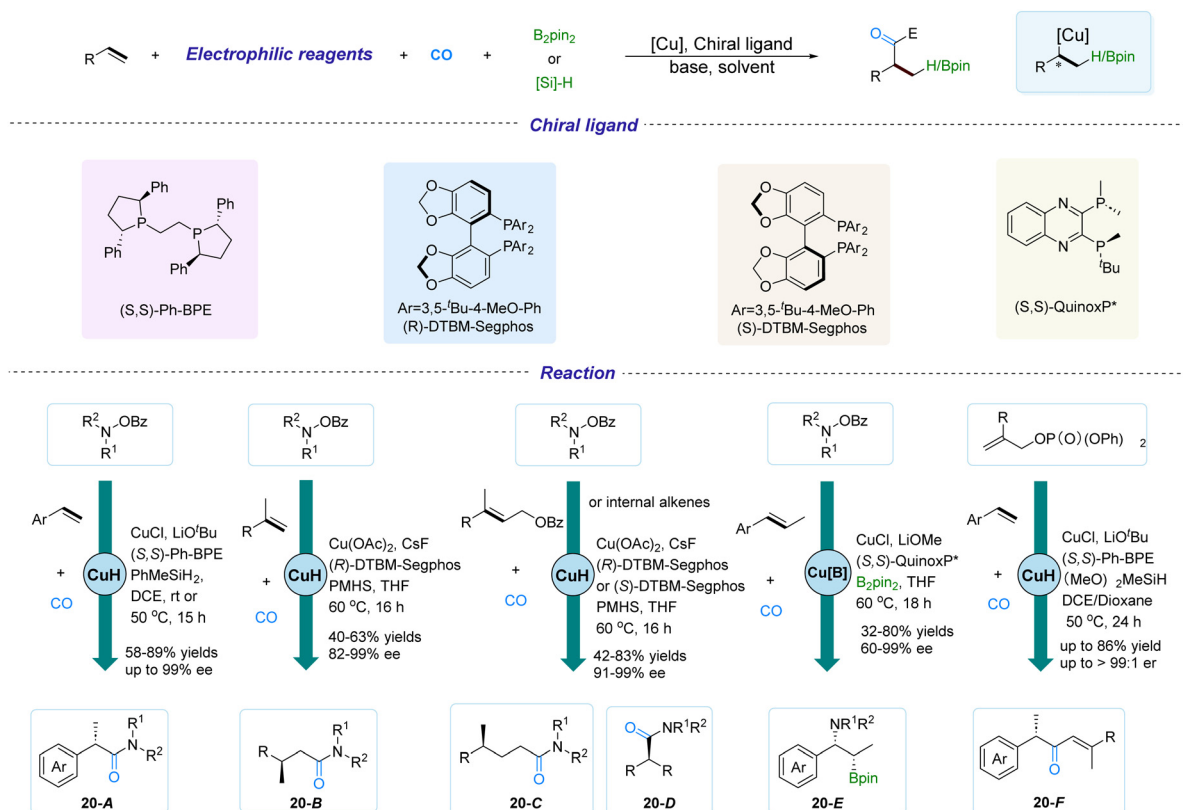
Fig. 20 Organocopper intermediates in the asymmetric carbonylative reaction (Cu–H and Cu–Bpin species addition to alkenes).
