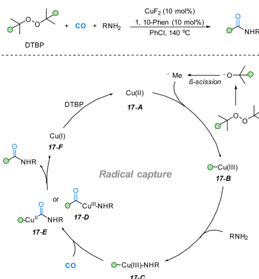
Fig. 17 Radical capture via \beta -scission toward acetamide derivatives.
