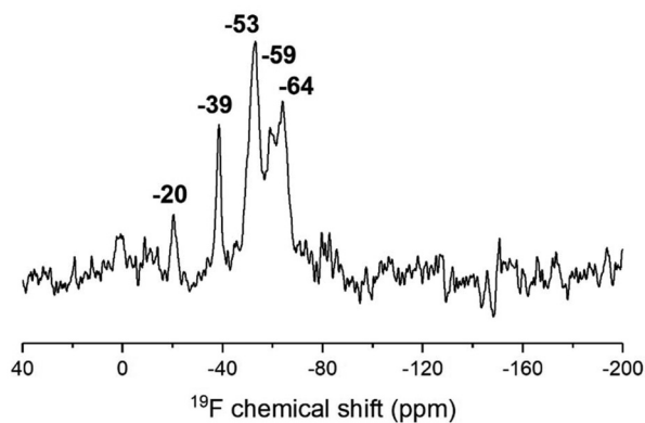
Fig. 8 ^{19}\text{F} MAS NMR spectrum of as-made EMM-17 using 8BMF as the OSDA at \text{Ge}_f 0.025. Resonances at -20 and -39 ppm correspond to types II and I, respectively, of F anions within d4r units while resonances at -53 , -59 , and -64 ppm are assigned to F anions confined within [4^35^4] cages.
