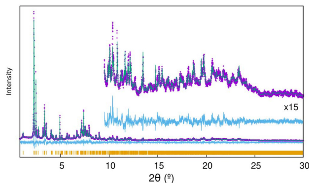
Fig. 5 Observed (purple +) and calculated (green solid line) synchrotron powder X-ray diffractograms for calcined HPM-9 refined in space group Pmmm . Vertical marks indicate the positions of allowed reflections. The cyan trace is the difference plot. The high angle region is also shown with expanded intensity (15×). \lambda = 0.49587 Å.
