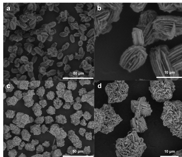
Fig. 10 Two typical morphologies found for EMM-17 synthesized using 8BMF: the rice of cards obtained at \text{Ge}_f = 0.025 (a and b) and the desert roses crystallized at \text{Ge}_f = 0.05 (c and d). In d, a TON impurity (as suggested by PXRD) is also observed.
