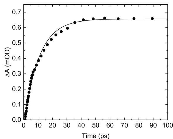
Fig. 6 The absorption trace recorded at 2341 \text{ cm}^{-1} associated with ground state \text{CO}_2 . The first 100 ps of the absorption trace is well described by a single exponential function with a time constant of \tau = 10.4 \pm 0.3 \text{ ps} .
