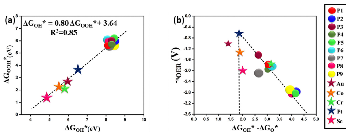
Fig. 8 (a) Scaling relations between \Delta G_{\text{OH}}^* and \Delta G_{\text{OOH}}^* ; (b) volcano curve between negative OER overpotential ( -\eta_{\text{OER}} ) and \Delta G_{\text{OH}}^* - \Delta G_{\text{O}}^* for HGY and TM@HGY.
